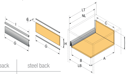
Inner drawer, height 94 and 126/218 mm
