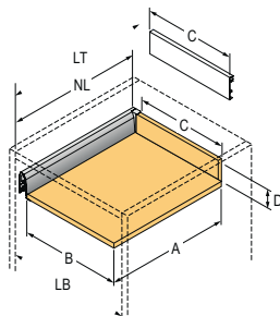
Inner drawer, height 94 mm
