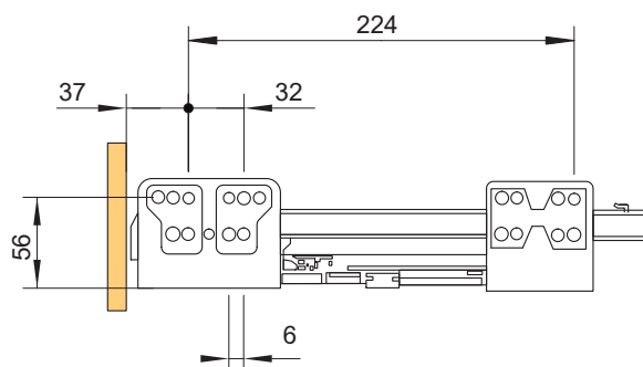
drilling holes for lengths 270 mm and 300 mm
