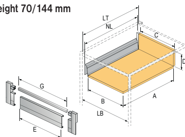
Inner drawer, height 70/144 mm
