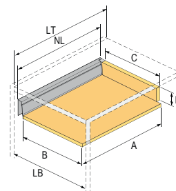
Front drawer, height 54 mm
