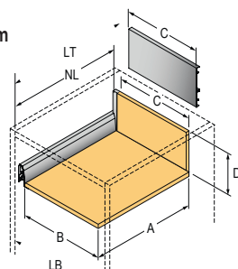
Front drawer, height 94 and 126/186 mm
