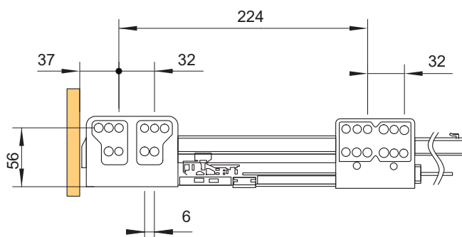
drilling holes for lengths from 350 mm to 550 mm
