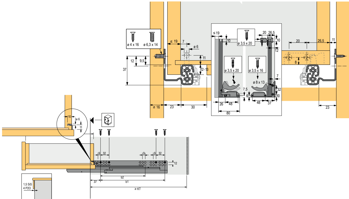
Quadro V6 full extension slide
