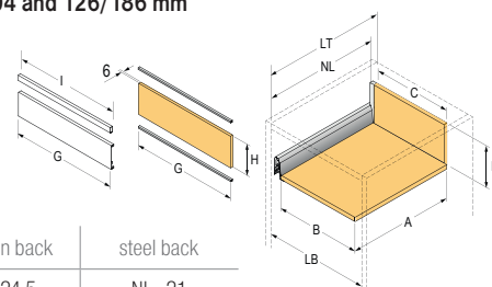
Inner drawer, height 94 and 126/186 mm
