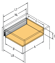
Inner drawer, height 126 mm
