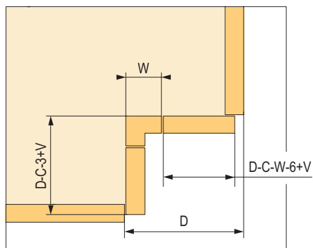
size of fronts with support
