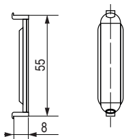
striker plate for rebate doors
