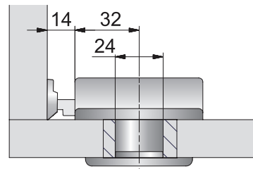
Darstellung geschlossen imaging closed
