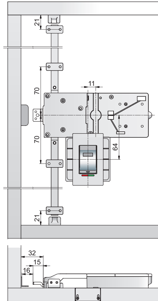
Drilling pattern / Bohrbild
