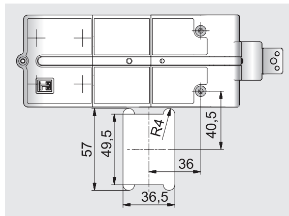
Drilling pattern / Bohrbild
